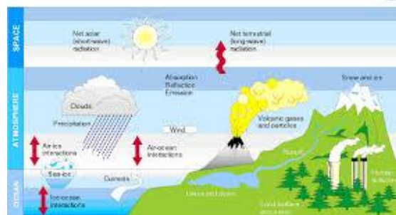
The Climate System
