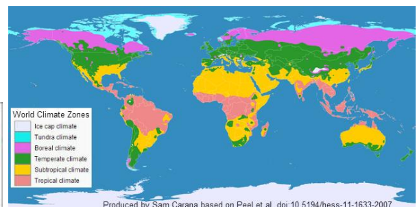
The Climate System
